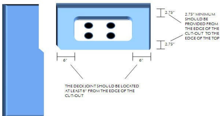
RECOMMENDED METHOD FOR INSTALLING HOT PLATES.
