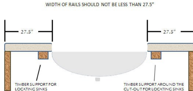
INSTALLATION OF UNDER THE COUNTER SINKS
