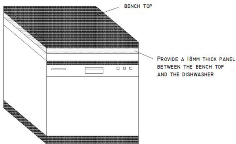
DISHWASHER INSTALLATION
